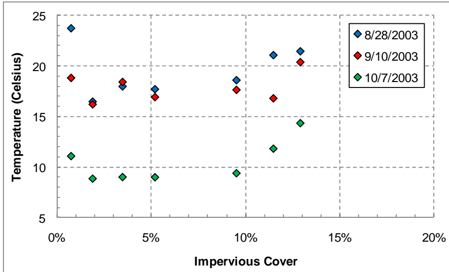
Figure E-1. Ohio EPA temperature grab samples from 2003.
